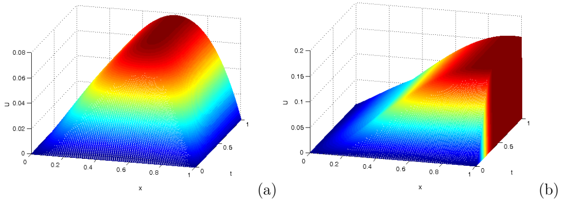
FIGURE 3. Example 4.1, (a) numerical solution for \varepsilon = 1 , \delta = 0.6\varepsilon and (b) numerical solution for \varepsilon = 2^{-10} , \delta = 0.6\varepsilon .
