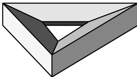
FIGURE 8. Cyclically piecewise convex polyhedron (1-toroid) T_9 with 9 vertices.
