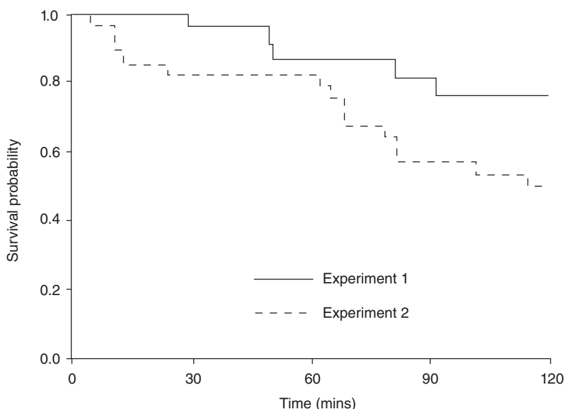
Figure 1.1. Example of a Kaplan–Meier curve. Taken from Altman (1991), Practical Statistics for Medical Research . Chapman and Hall/CRC, p. 374.
