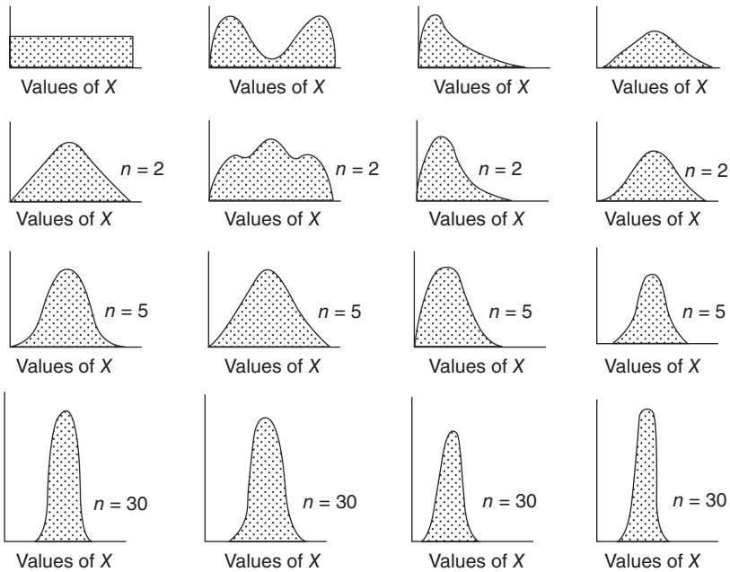
Figure 4.1. The effect of shape of population distribution and sample size on the distribution of means of random samples. Source: Kuzma, J. W. (1984). Basic Statistics for the Health Sciences . Mountain View, CA: Mayfield Publishing Company, figure 7.2, p. 82.
